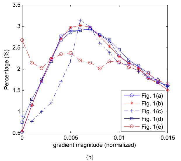
Fig. 2. (a) Histograms of the Gaussian-smoothed gradient components (including both I_h and I_v ) computed from the five images shown in Fig. 1. (b) Histograms of the gradient magnitudes computed from the five Gaussian-smoothed images shown in Fig. 1.
