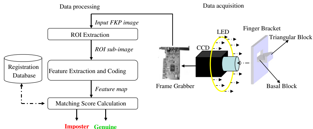
Fig. 1. Structure of the proposed FKP-based personal authentication system. The whole system is composed of a data acquisition module and a data processing module.
