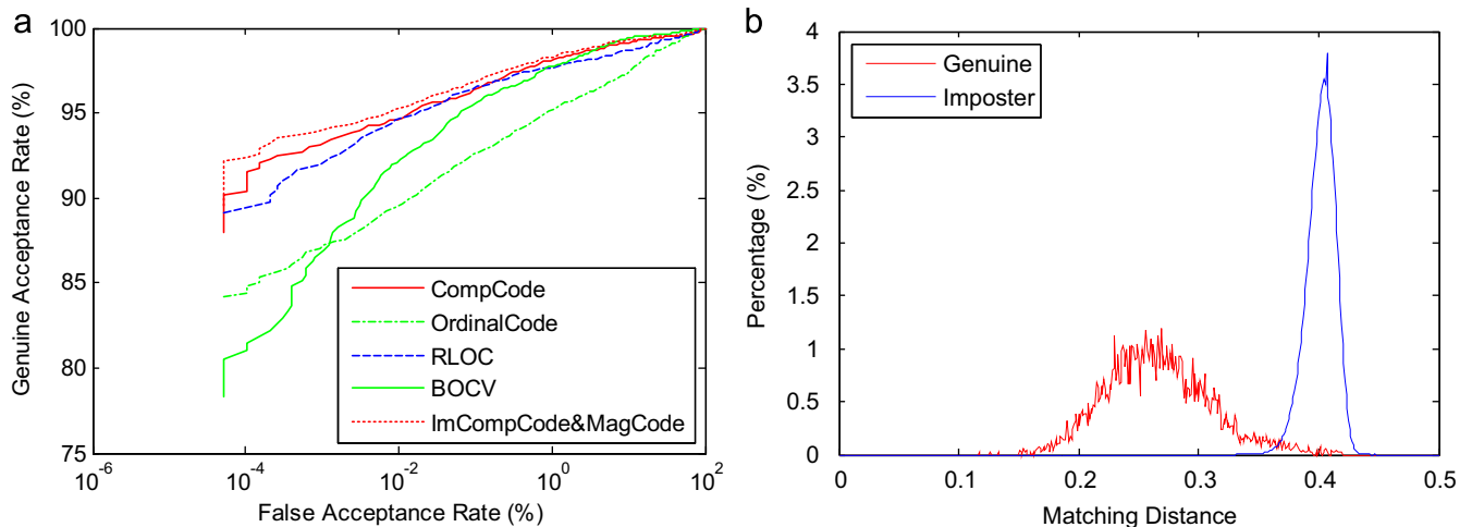
Fig. 8. (a) ROC curves obtained by five recognition methods in experiment 1 and (b) distance distributions of genuine matchings and imposter matchings with the proposed scheme in experiment 1.
