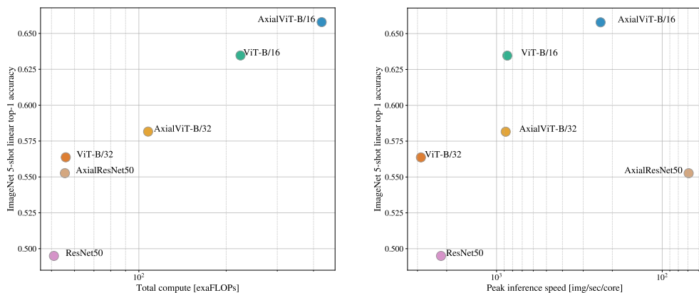
Figure 12: Performance of Axial-Attention based models, in terms of top-1 accuracy on ImageNet 5-shot linear, versus their speed in terms of number of FLOPs ( left ) and inference time ( right ).
