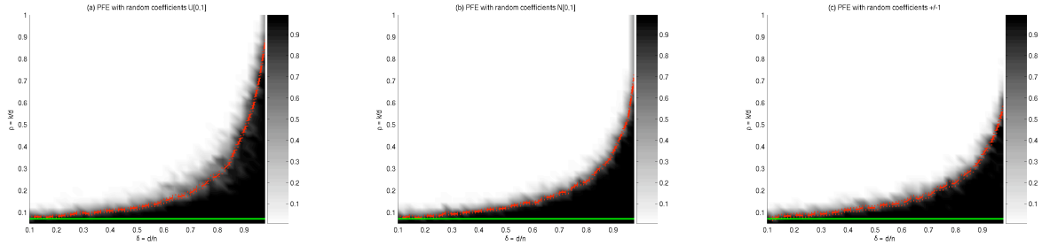
Figure 8: k -Step Solution Property of HOMOTOPY for the Suite \mathcal{S}(\text{PFE}, \mathbf{V}; d, n, k) . Each phase diagram presents success rates on a \rho - \delta grid, with \rho = k/d in [0.05, 1] , \delta = d/n in [0.1, 1] , and n = 1024 , for: (a) \mathbf{V} = \text{UNIFORM} ; (b) \mathbf{V} = \text{GAUSS} ; (c) \mathbf{V} = \text{BERNOULLI} . Overlaid are curves for \hat{\rho}_{0.25}(\delta) (dash-dotted), with the confidence bounds for 95% confidence level (dotted), and \rho = 1/(2 \log(n)) (solid). The range of sparsities in which the k -step solution property holds is much more extensive than implied by the bound k < d/(2 \log(n)) .
